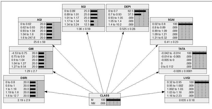
Figure 2: Learned-training Data Set Using EM Algorithm – The BNC Network
