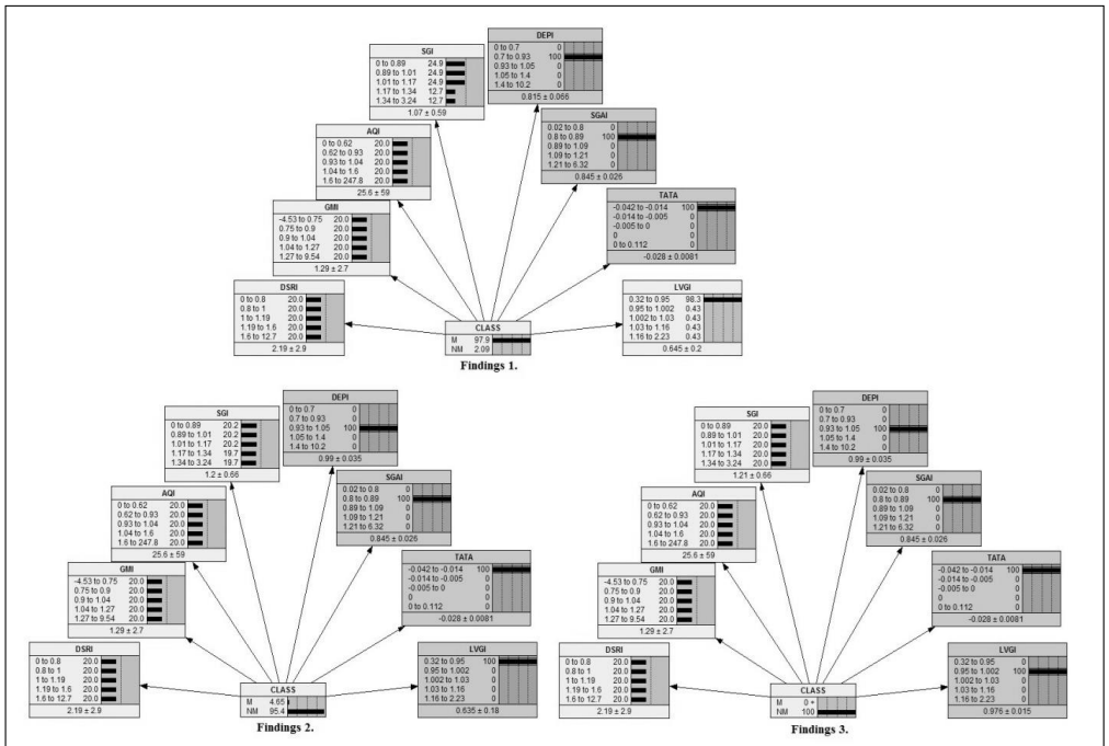
Figure 4: Sample Findings of DEPI, SGAI, TATA and LVGI - The BNC Network
