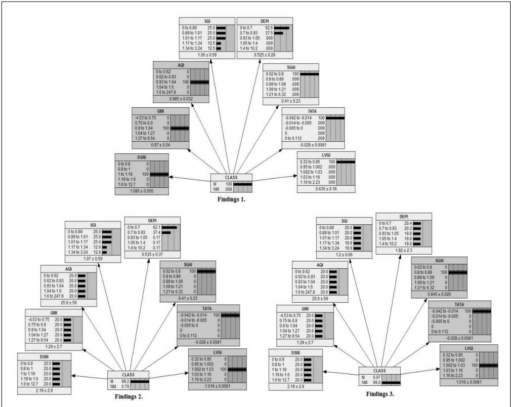
Figure 3: Sample Findings of AQI, GMI, DSRI, SGAI, TATA and LVGI - The BNC Network
